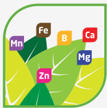
BORON ETHANOLAMINE
